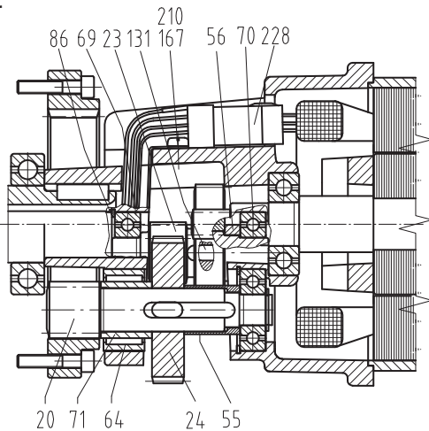
3-stage gearbox
