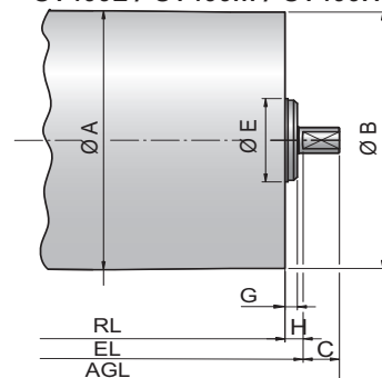
Idler Pulley UT400L / UT400M / UT400H
