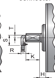
Elbow connector
