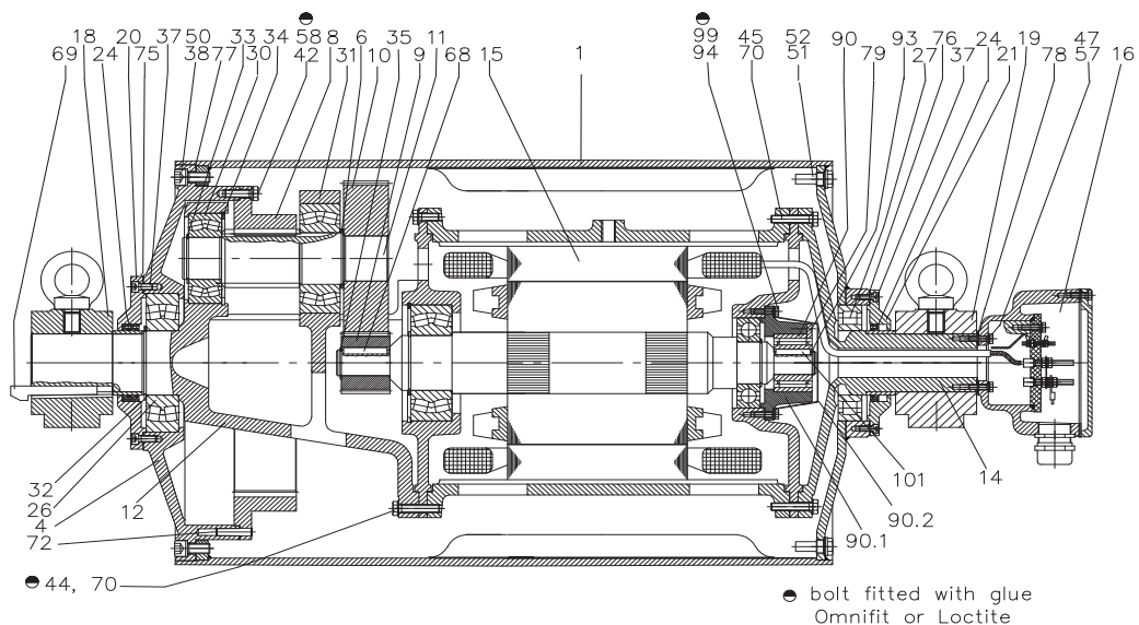
Backstop Execution
