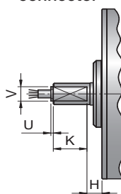
Straight connector
