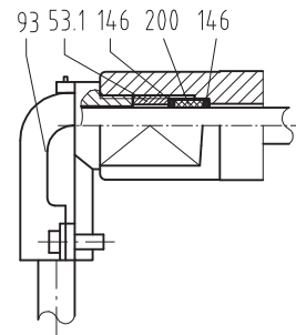
Cable version with elbow connector
