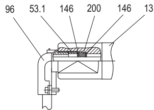
Elbow Connector
