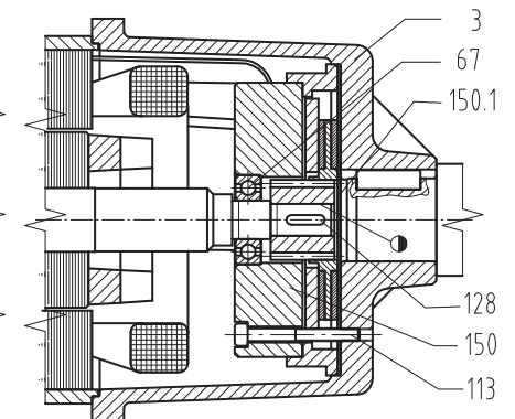
Electromagnetic brake
