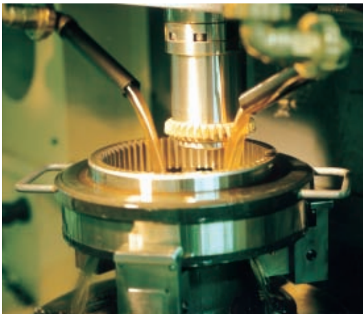
CNC gear shaping machine
